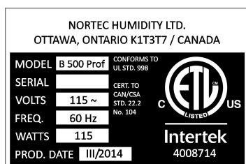
Fig. 75: Type plate
