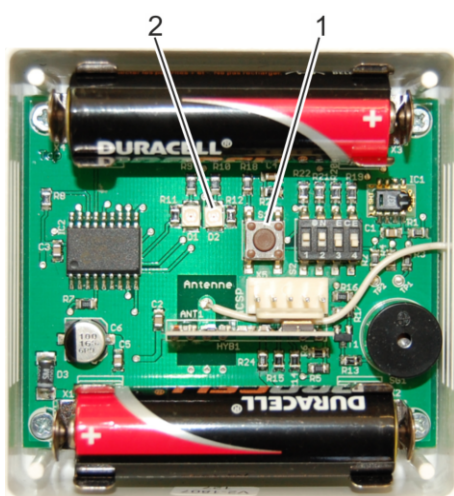
Fig. 13: Check functionality
