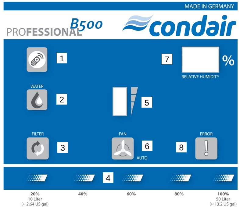
Fig. 5: Control panel
