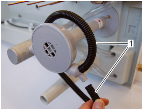
Fig. 38: Take off pump hoses
