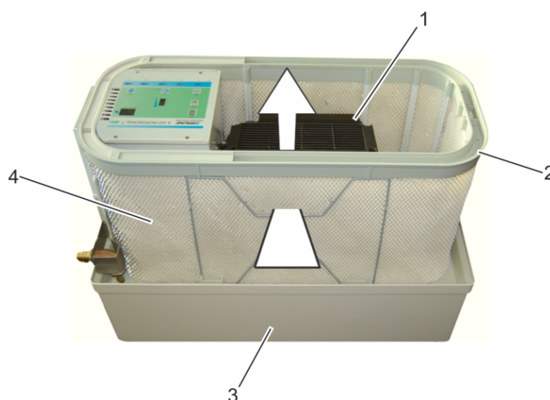
Fig. 6: Functional principle
