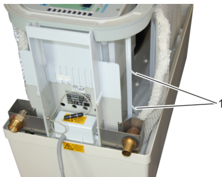
Fig. 31: Fasten filter
